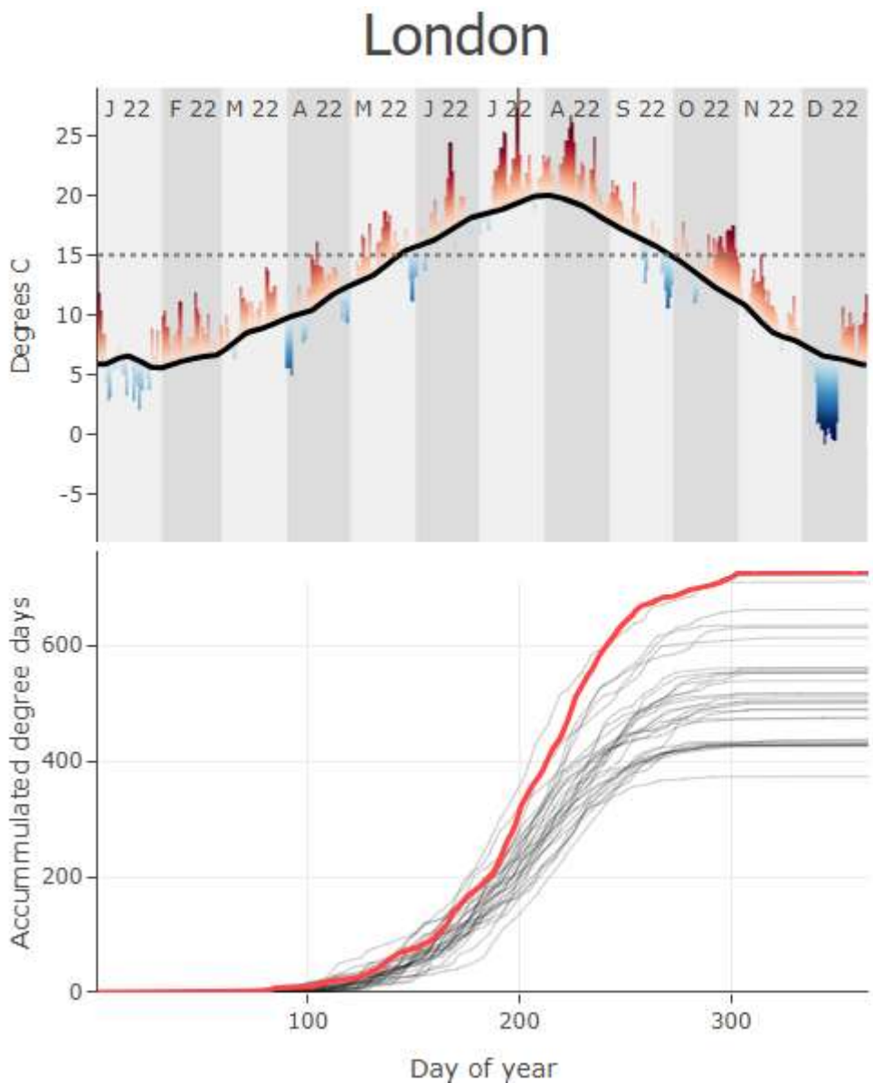
Fig. 4 Top graph shows the recorded air temperatures for London (one of the warmest parts of the UK) during 2022 (the warmest year on record). The dotted line at 15°C is the lower developmental threshold temperature (LDT) for the larval stage of D. abbreviatus (only June, July, August and September had mean temperatures above the LDT). Bottom graph shows the degree days that would have been accumulated (red line = in London in the year of 2022, grey lines = degree day accumulations for different years in London) had the larval stage commenced development on the 1 st of January and its environmental temperature been equal to air temperature – the larval stage would be developing below ground where temperatures would be buffered in comparison to air
