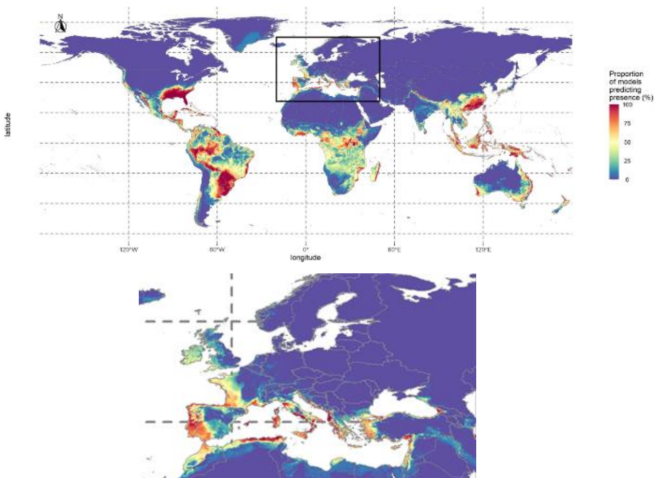
Figure 1. Maps showing habitat suitability of Xylosandrus compactus under current climate conditions. This consensus map was computed by averaging binary maps and represents the percentage of models predicting each pixel as suitable. The black square represents the limits of the focal area - the second map is the same area zoomed in. Produced by Urvois et al. (2021a) CC BY 4.0
